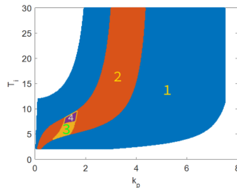
Fig. 1 - Visualization of the change in the zone of possible tunings depending on the search area: 1 - rational constraints only, 2 - constraints on PM , 3- constraints on PM & u_{max} , 4 - constraints on PM & u_{max} & M_p
